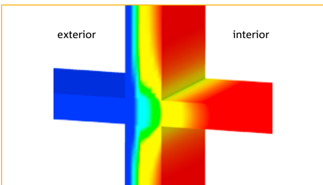
Thermal bridging allows freezing temperatures to flow into the building creating cold floors and higher electricity costs.
